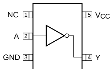
Figure 3. SC70 (Top View)
