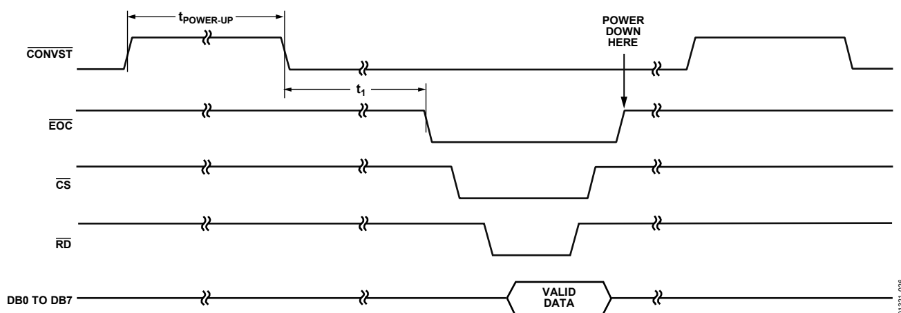
Figure 25. Mode 2 Operation
