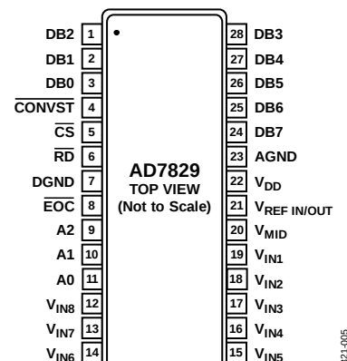
Figure 5. Pin Configuration
