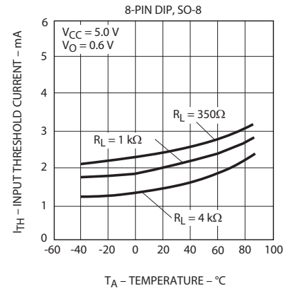
Figure 3: Typical Input Threshold Current vs. Temperature
