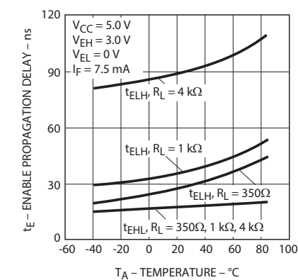
Figure 14: Typical Enable Propagation Delay vs. Temperature
