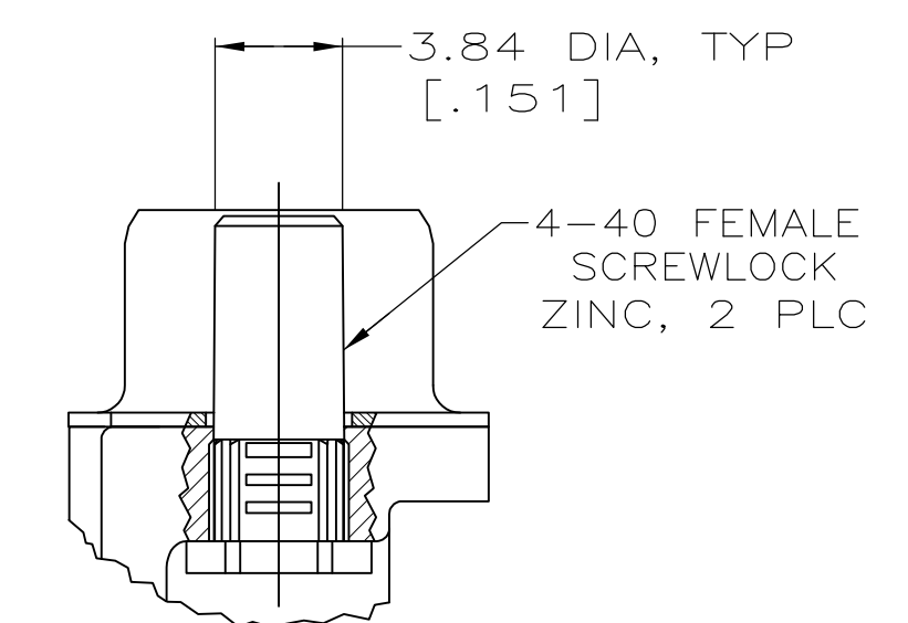
DETAIL E
