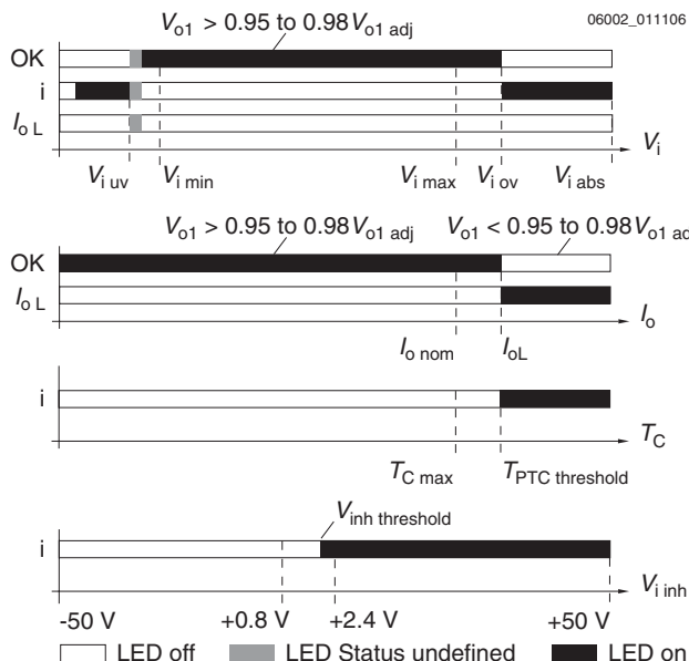
Fig. 18 LED indicators
