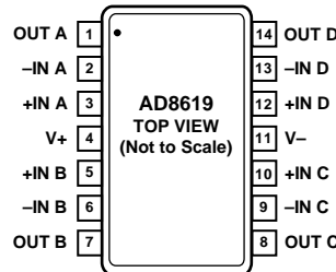
Figure 4. 14-Lead TSSOP
