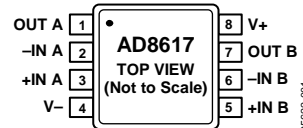
Figure 2. 8-Lead MSOP and 8-Lead SOIC_N
