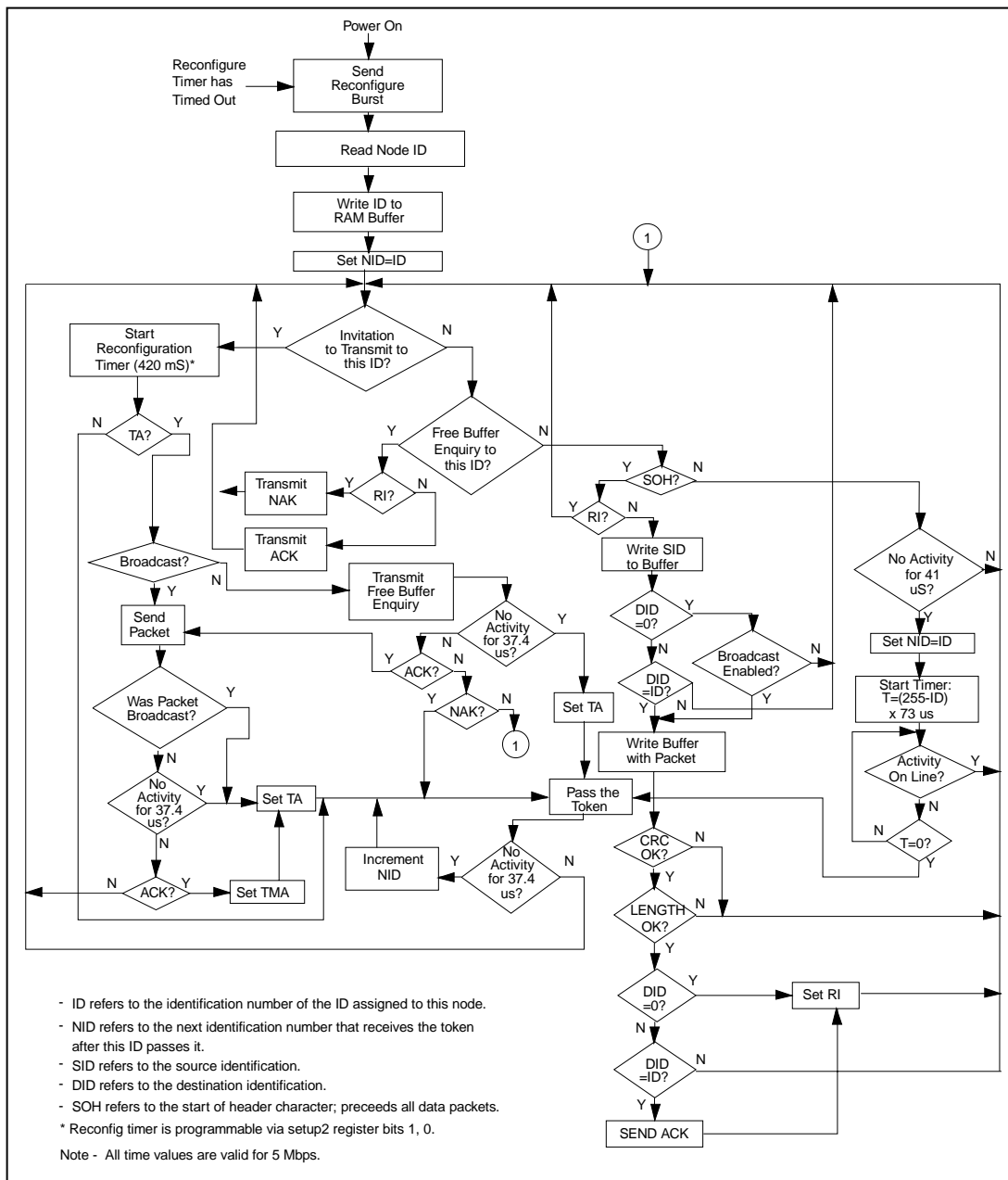
FIGURE 1 - COM20020I OPERATION
