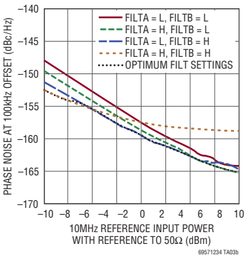
Additive Phase Noise vs Input Amplitude
