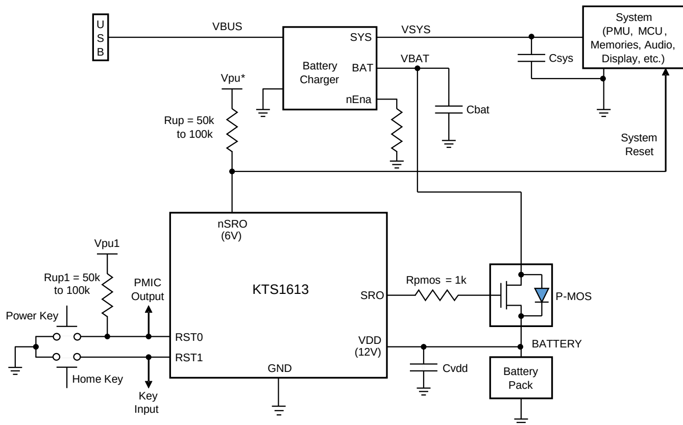
Figure 4. Application Circuit
