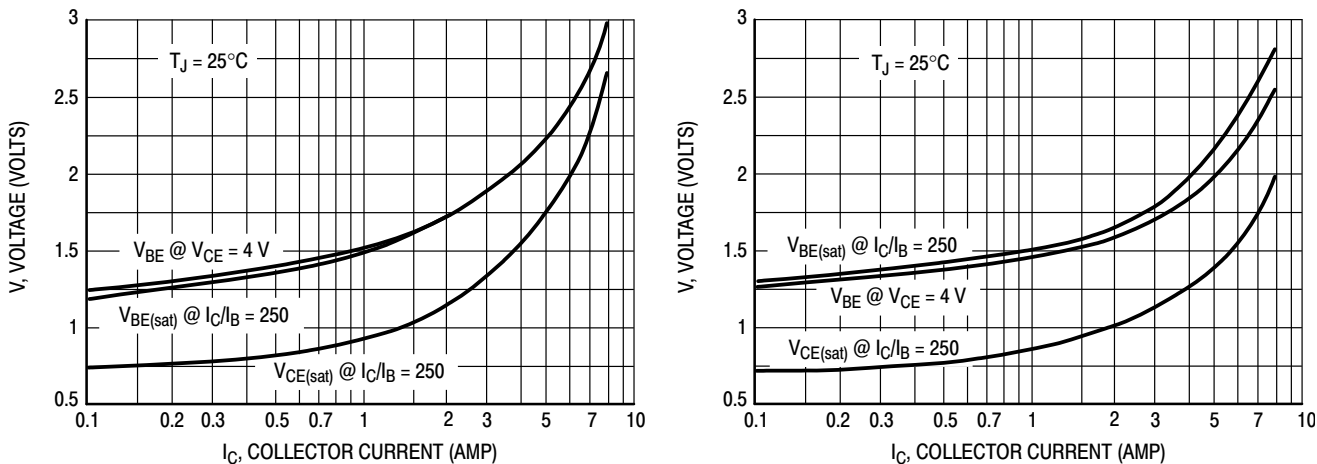
Figure 4. "On" Voltages
