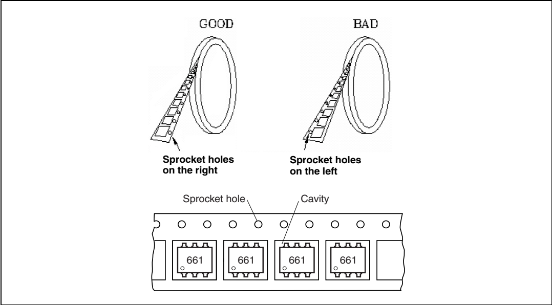
Figure 20. Device orientation
