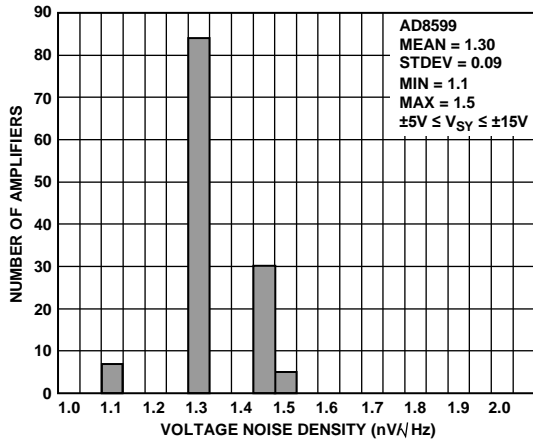
Figure 40. Voltage Noise Density @ 10 Hz
