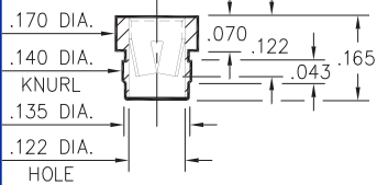
0388-0-15-XX-08-XX-10-0 Press-fit in .138 mounting hole
