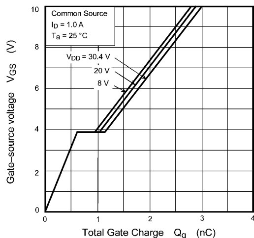
Fig. 7.11 Dynamic Input Characteristics
