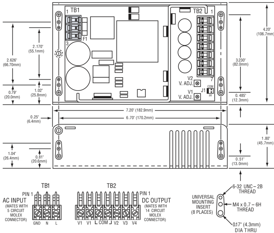
Figure 1. Mechanical Drawing
