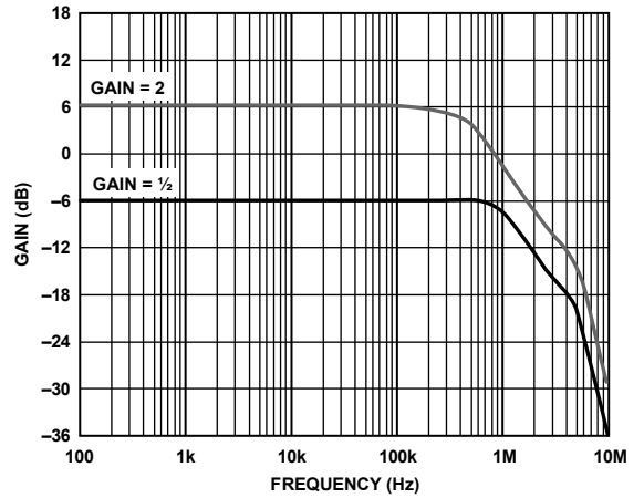
Figure 18. Gain vs. Frequency, \pm 15V Supplies
