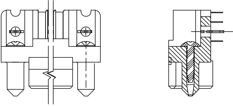
SECTION U-U
