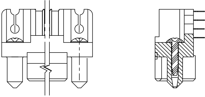
SECTION U-U
