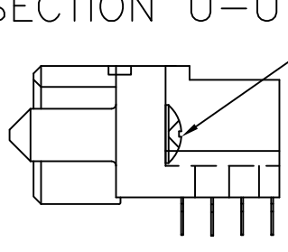
SECTION U-U
