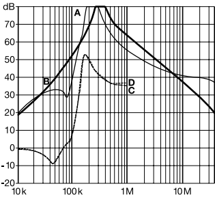
230 A types
