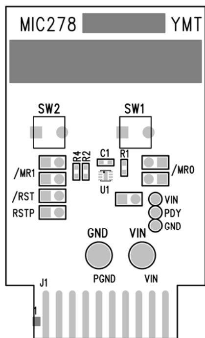
Top Silkscreen
