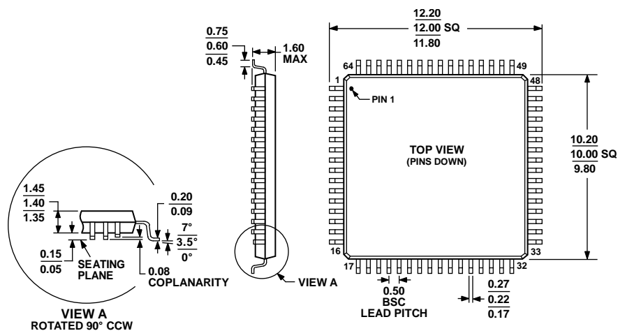
Figure 44. 64-Lead Low Profile Quad Flat Package [LQFP] (ST-64-2)
