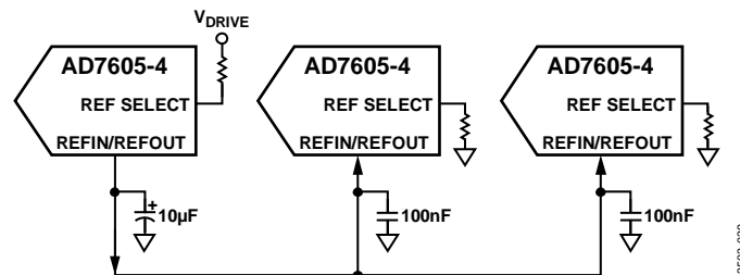
Figure 36. Internal Reference Driving Multiple AD7605-4 REF OUT Pins
