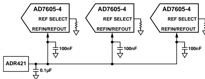
Figure 35. Single External Reference Driving Multiple AD7605-4 REF OUT Pins
