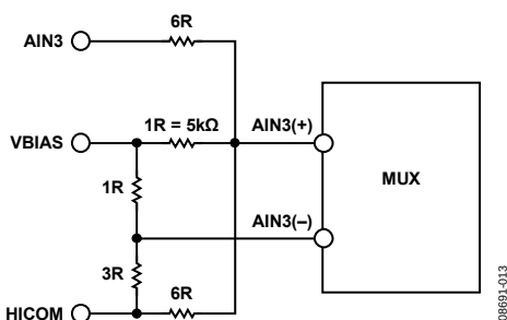
Figure 13. AIN3 Input Structure
