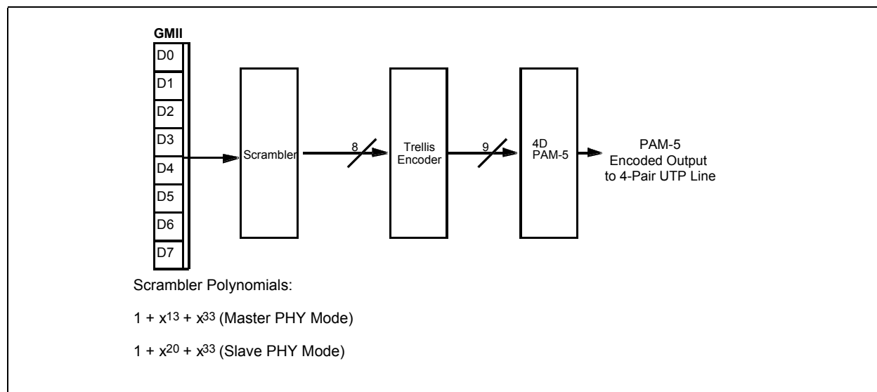
Figure 3-8. 100BASE-T Transmit Flow And Line Coding Scheme
