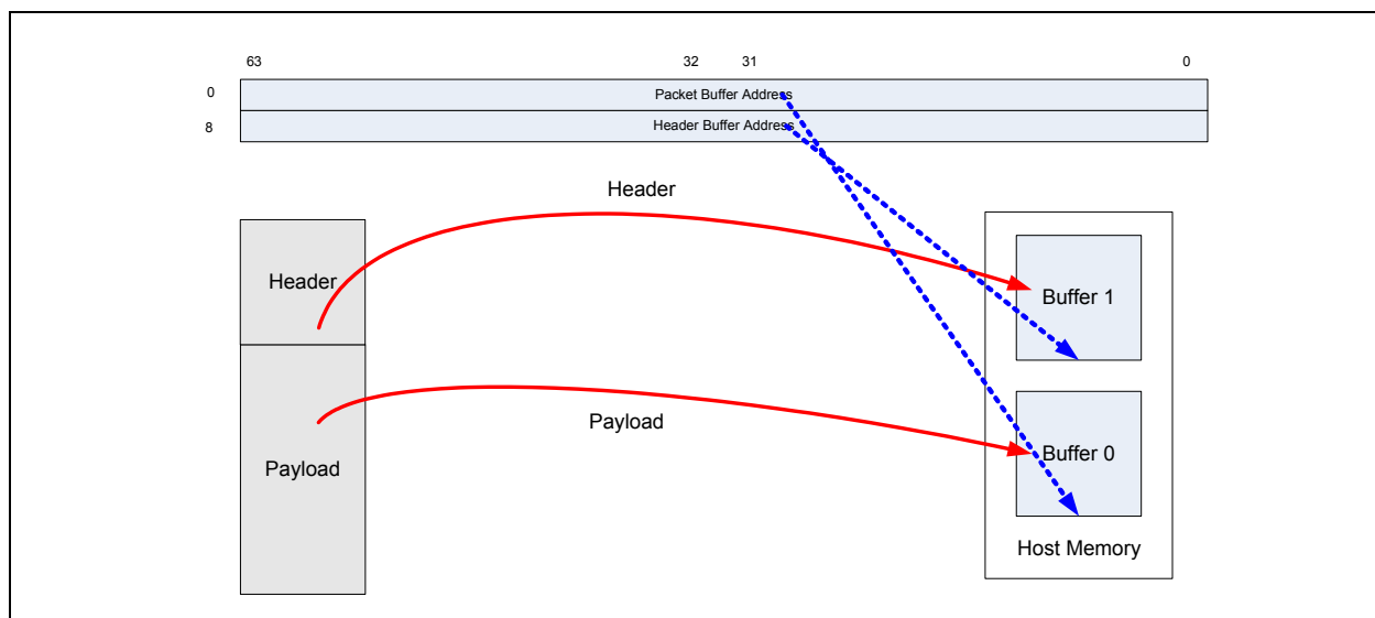
Figure 7-10. Header Splitting
