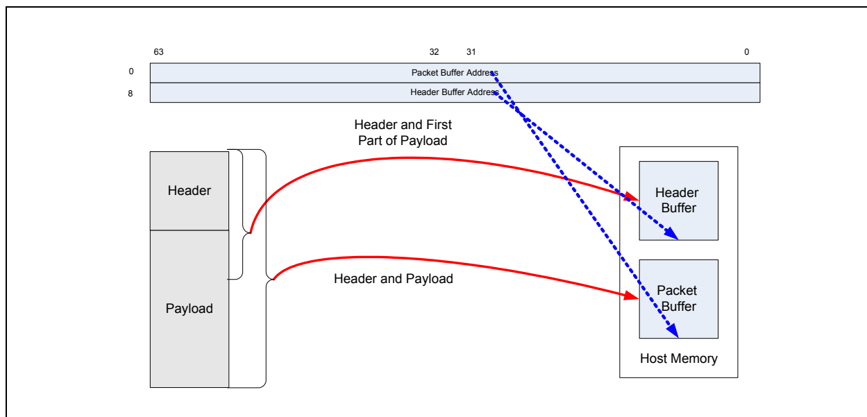
Figure 7-11. Header Replication
