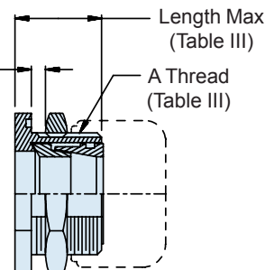
Style 1 - RFI/EMI Type A - Rear Mount
