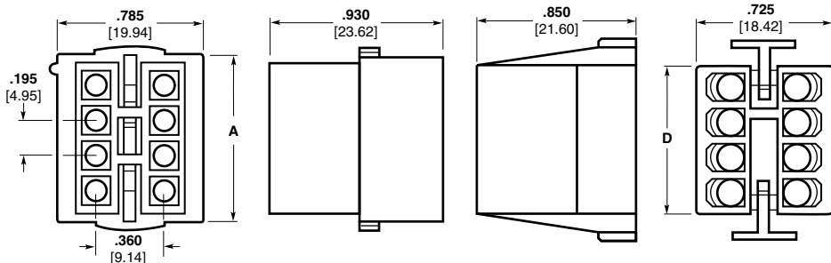
Pin Housing (Cap)
