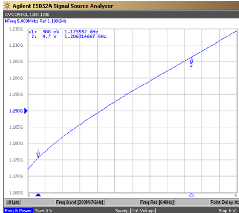
Tuning Curve (Typical)
