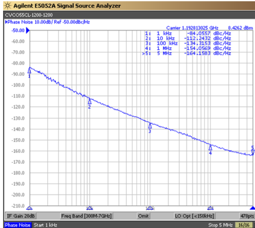
Phase Noise (1 Hz BW, Typical)
