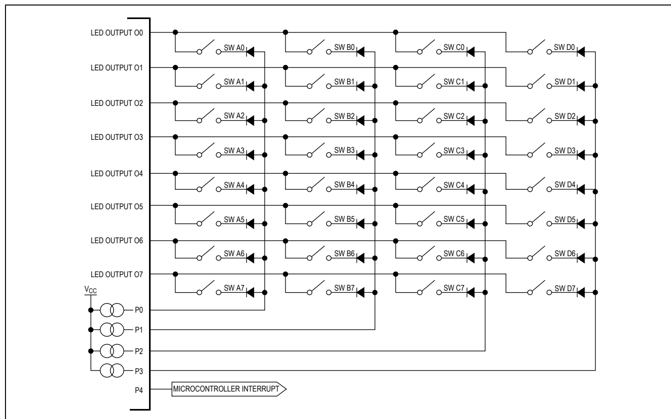
Figure 7. Key-Scanning Configuration
