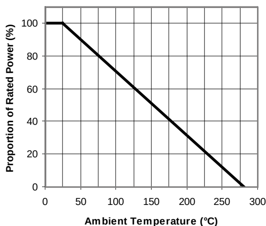
Derating Curve
