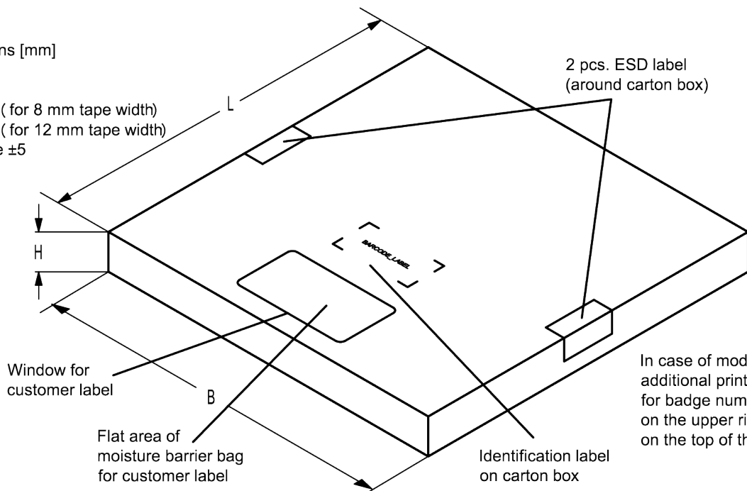
Figure 18: Drawing of folding box for reel with diameter of 330 mm.
