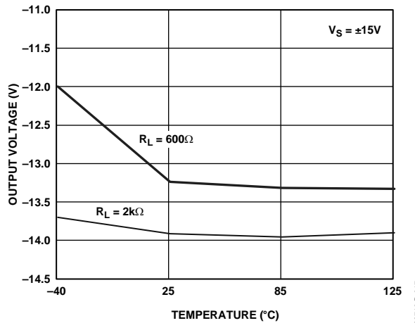
Figure 15. Output Voltage Low vs. Temperature
