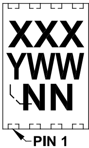
8-Lead TDFN (2x3) (MCP9844)
