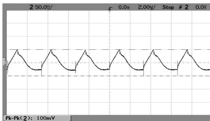
Output Ripple and Noise (V IN =12V, V OUT =3.3V, I OUT =16A, C LOAD =0, ScopeBW=100MHz)
