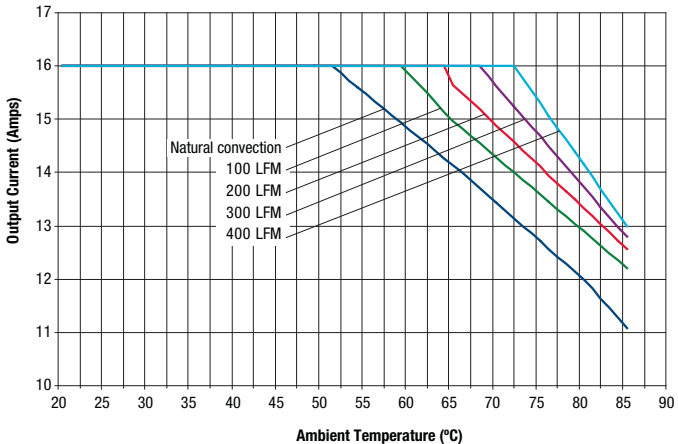
OKY2-T/16-D12-C Maximum Current Temperature Derating at Sea Level (V IN = 12V, V OUT = 0.75V).
