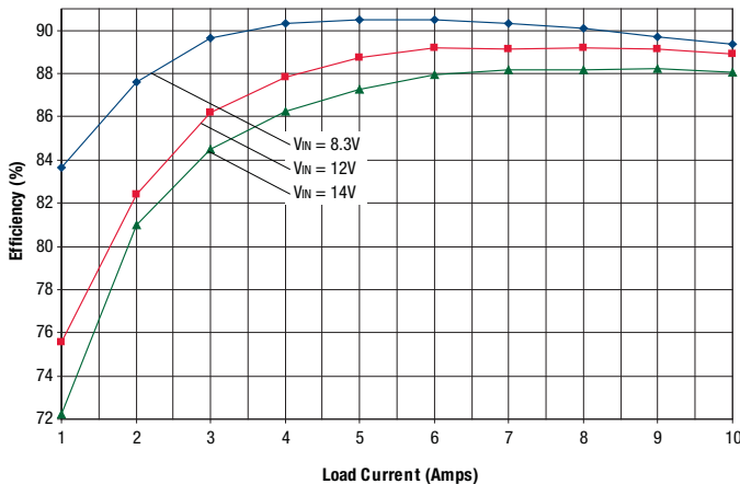
OKY2-T/10-D12 Efficiency vs. Line Voltage and Load Current @ +25°C (V OUT = 1.8)
