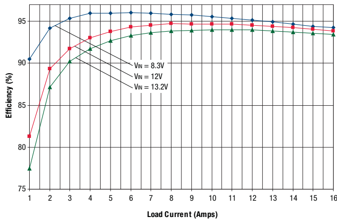
OKY2-T/16-D12 Efficiency vs. Line Voltage and Load Current @ +25°C (V OUT = 5V)
