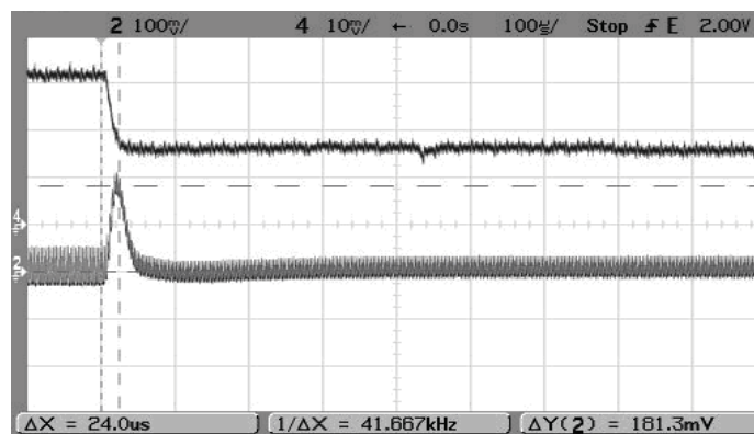
Step Load Transient Response (V IN =12V, V OUT =3.3V, C LOAD =0, I OUT =16A to 8A) Trace 2=V OUT , 100 mV/div, Trace4=I OUT , 5A/div.
