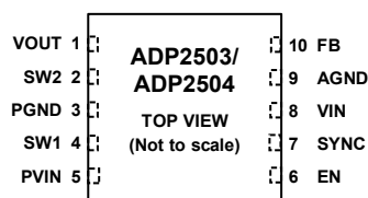
Figure 2. Pin Configuration
