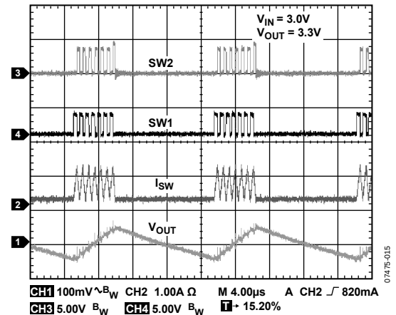
Figure 25. Typical PSM Switching Waveform, Buck-Boost Operation ( V_{OUT} = 3.3 V)
