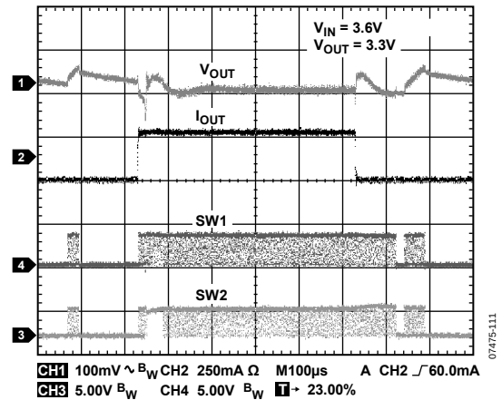
Figure 19. Load Transient ( V_{IN} = 3.6V , V_{OUT} = 3.3V , I_{OUT} = 10mA to 300mA )
