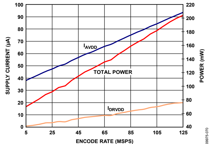
Figure 59. AD9648-125 Power and Current vs. Clock Rate (1.8 V CMOS Output Mode)
