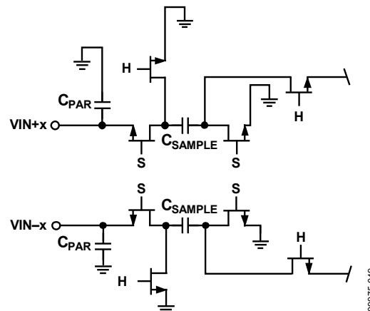
Figure 42. Switched-Capacitor Input Circuit
