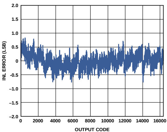
Figure 22. INL Error with f_{IN} = 9.7 MHz
