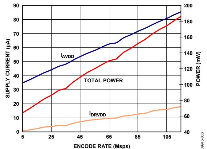
Figure 60. AD9648-105 Power and Current vs. Clock Rate (1.8 V CMOS Output Mode)
