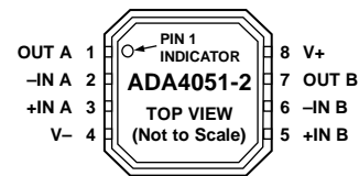
Figure 4. 8-Lead LFCSP (CP-8-2)
