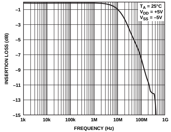
Figure 20. On Response vs. Frequency
