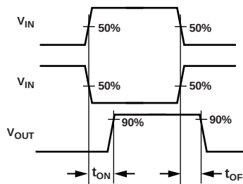
Figure 30. Switching Times
