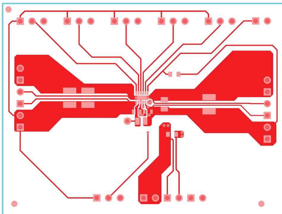
Figure 4. Top Layer
