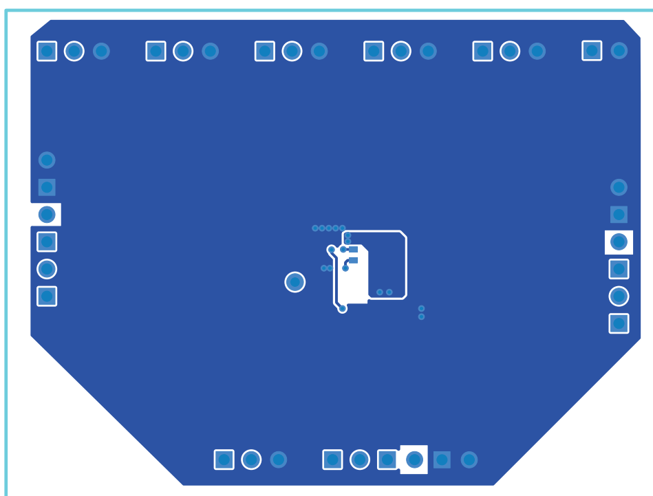
Figure 5. Bottom Layer
