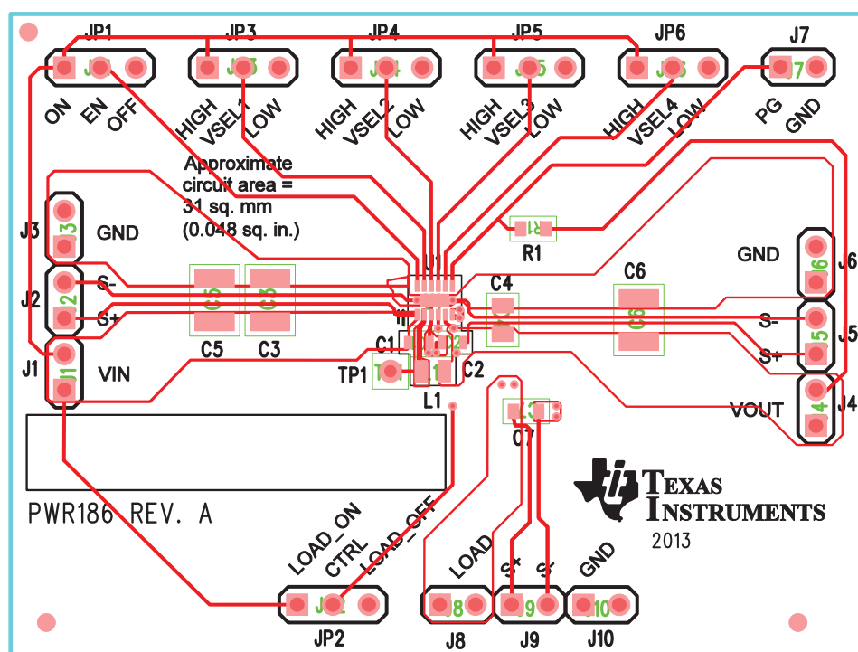
Figure 2. Assembly Layer
