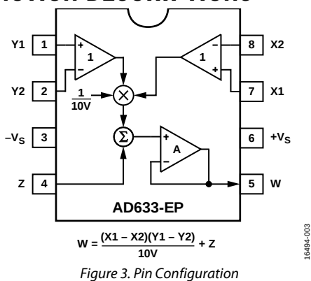
Figure 3. Pin Configuration
