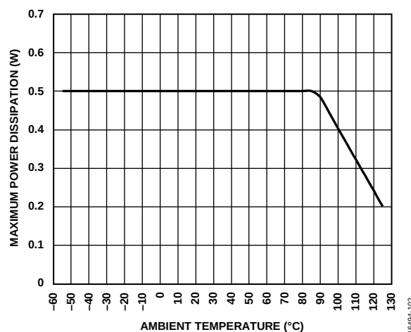
Figure 2. Maximum Power Dissipation vs. Ambient Temperature ( T_A )
