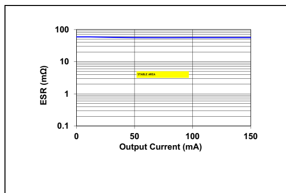
FIGURE 2-41: ESR vs. Load - LDO2.
