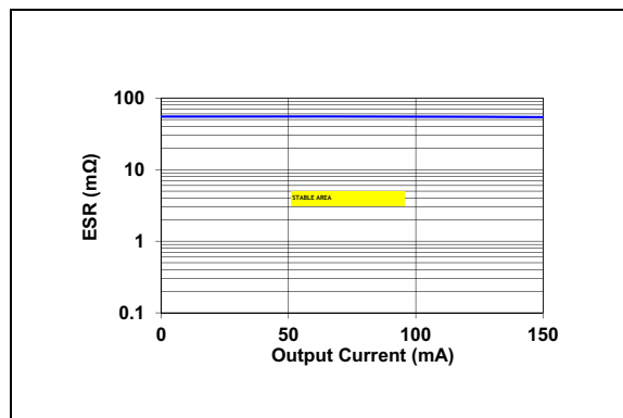
FIGURE 2-40: ESR vs. Load - LDO1.
