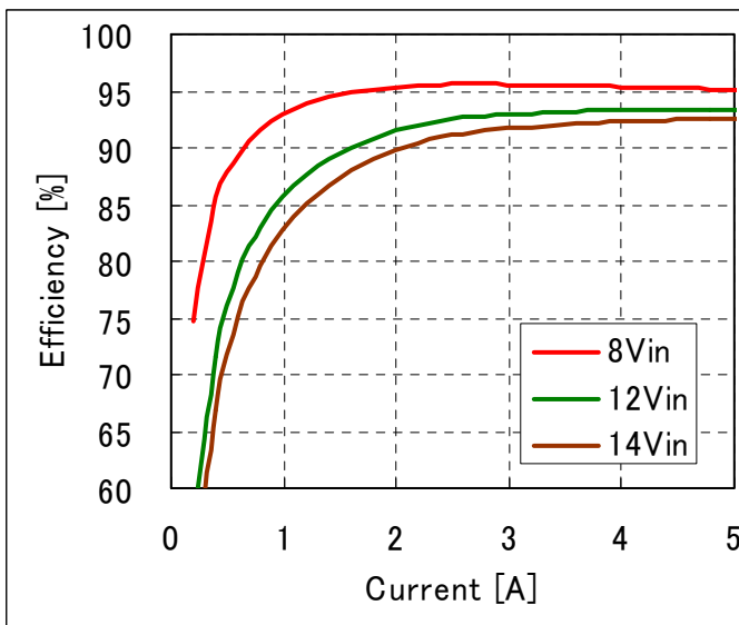
Fig-5.0V-2: Efficiency vs. load current and input voltage for V_{out}=5.0V . Airflow rate=200 LFM (1m/s) and T_a=25^{\circ}C .
