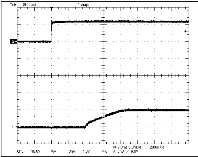
Fig-1.0V-4: Turn-on transient for V_{out}=1.0V with application of V_{in} at full rated load current (resistive) and 47\mu F \times 2 external capacitance at V_{in}=12V .
