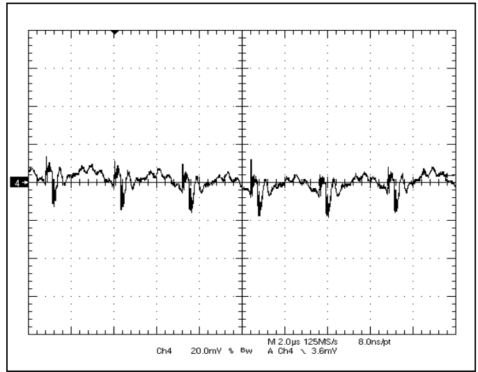
Fig-1.0V-5: Output voltage ripple (20mV/div.) for V_{out}=1.0V at full rated load current into a resistive load with external capacitance 47\mu F \times 2 ceramic + 1\mu F ceramic at V_{in}=12V .
