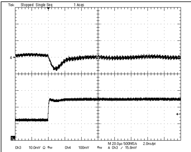
Fig-1.0V-6: Output voltage response for V_{out}=1.0V to positive load current step change from 2.5A to 5A with slew rate of 5A/\mu s at V_{in}=12V . C_o=47\mu F \times 2 ceramic.
