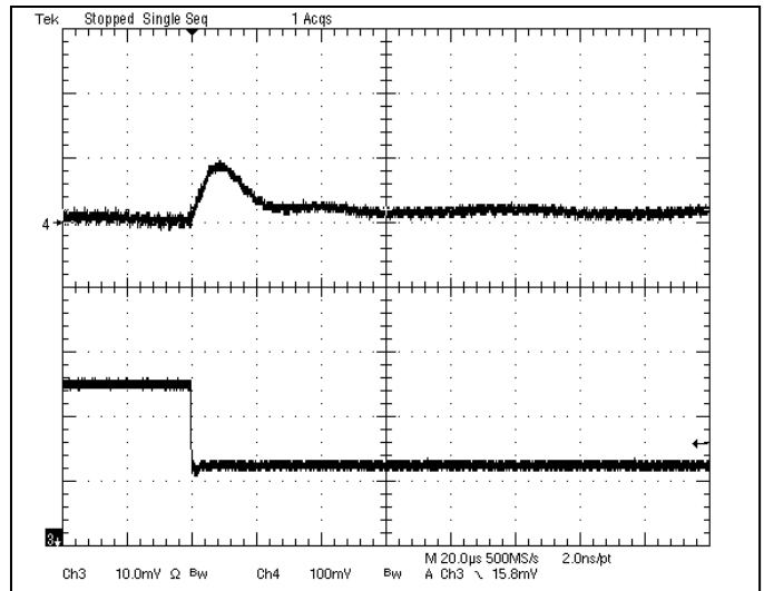
Fig-1.0V-7: Output voltage response for V_{out}=1.0V to negative load current step change from 5A to 2.5A with slew rate of -5A/\mu s at V_{in}=12V . C_o=47\mu F \times 2 ceramic.
