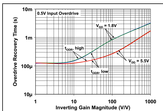
FIGURE 2-50: Output Overdrive Recovery Time vs. Inverting Gain.
