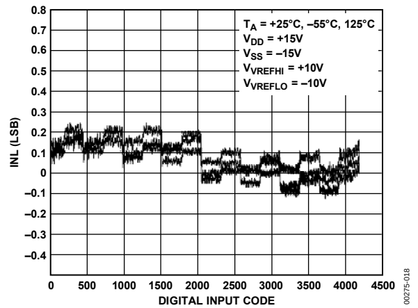
Figure 17. INL vs. Code
