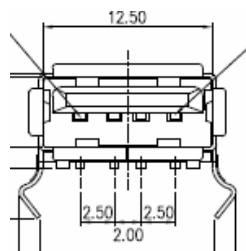
A Type Standard Board Lock SMT
