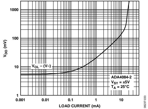
Figure 37. Dropout Voltage vs. Sink Current
